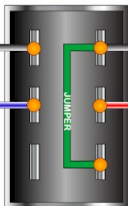
DP (ON-OFF-ON) Switch (Rear View) Wired for:
